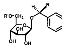
Gentiobioside Series (R' = \beta -D-glucopyranosyl)
